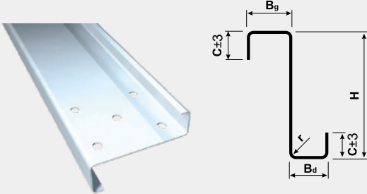
Z-profiel
