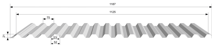
Sormonto una greca 1 rib overlap
