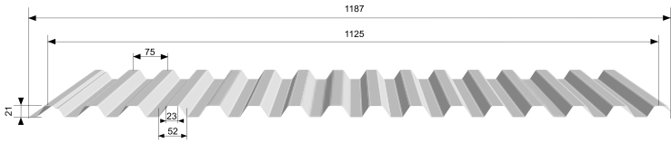
Sormonto una greca 1 rib overlap
