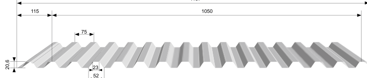
Sormonto due greche 2 ribs overlap
